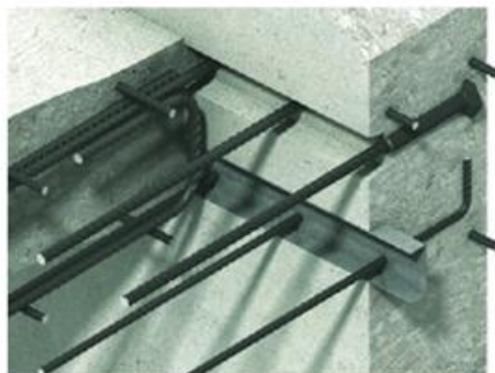
KSN Anchor System being used with an Eazistrip System
