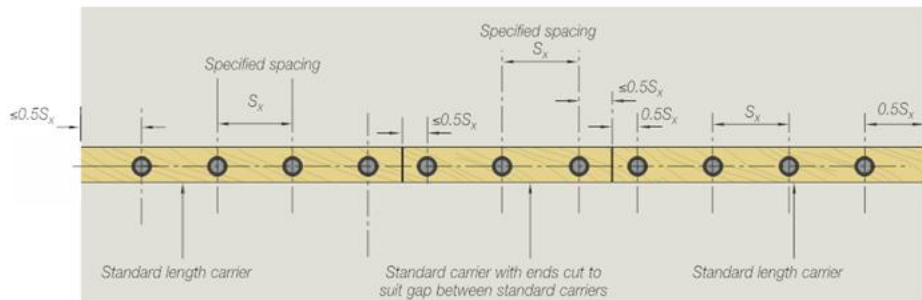
Wall Elevation
