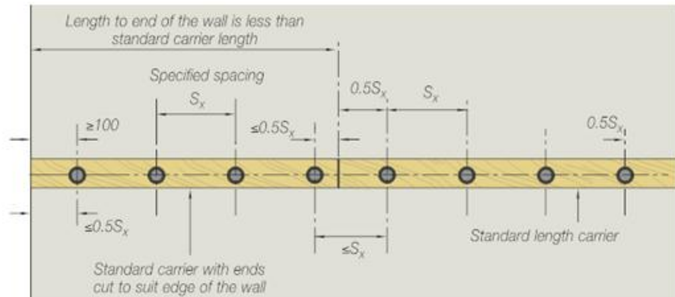
Wall Elevation
