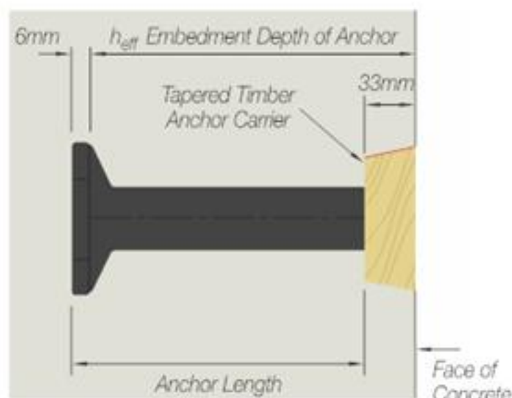
Anchor Embedment Arrangement
