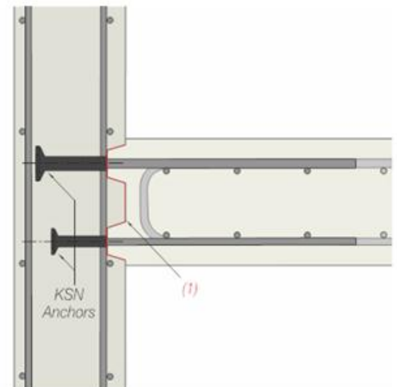
Wall/Slab Section - KSN Anchors
