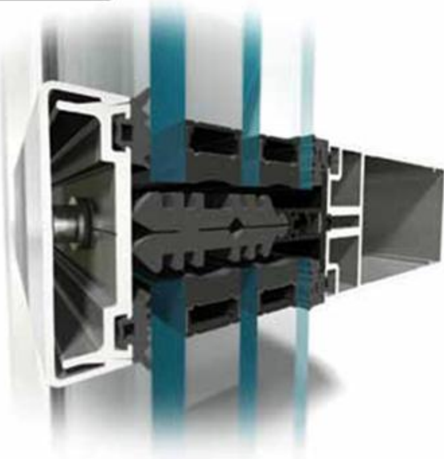
Transom - cross section
